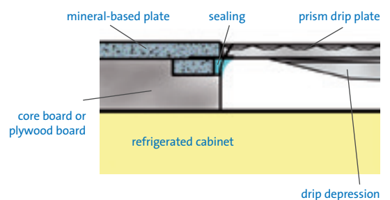
cross section supporting plate / drip tray (bottom side assembly)
