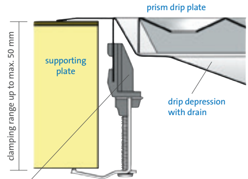
cross section supporting plate / drip tray (top side assembly)
